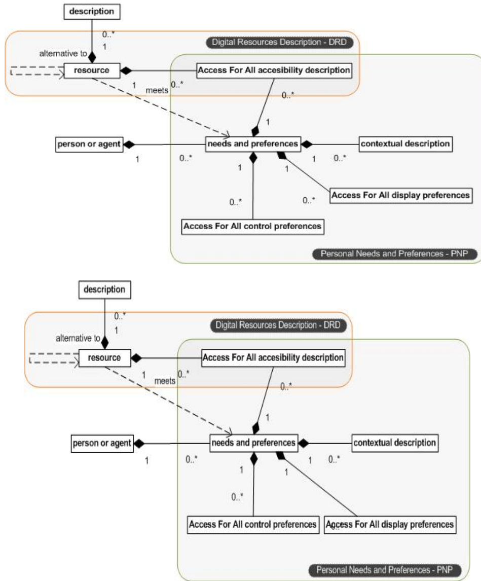
Fig. 1. Access For All Abstract Model [6]
