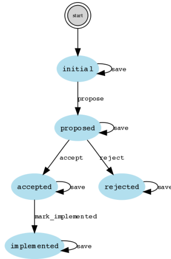
Fig. 3. State Graph for the TIP Workflow
