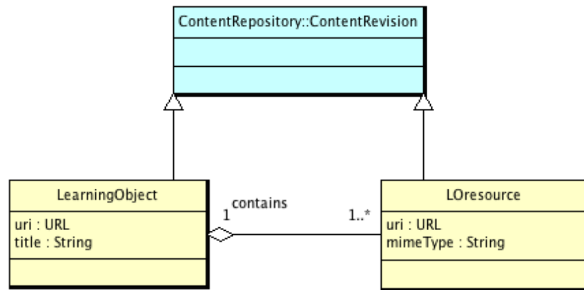
Fig. 2. OpenACS learning object content type model
